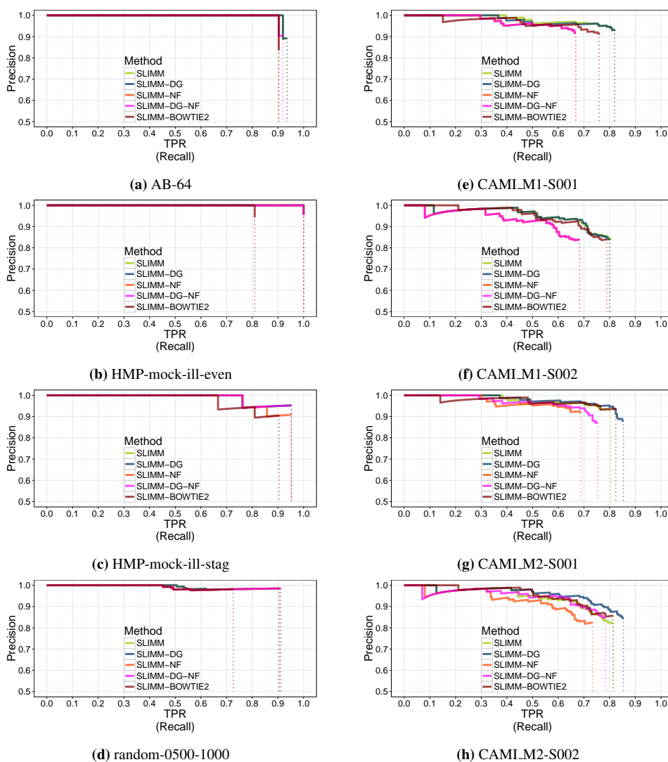
Figure 2. Precision - Recall Curves: Different SLIMM variants
