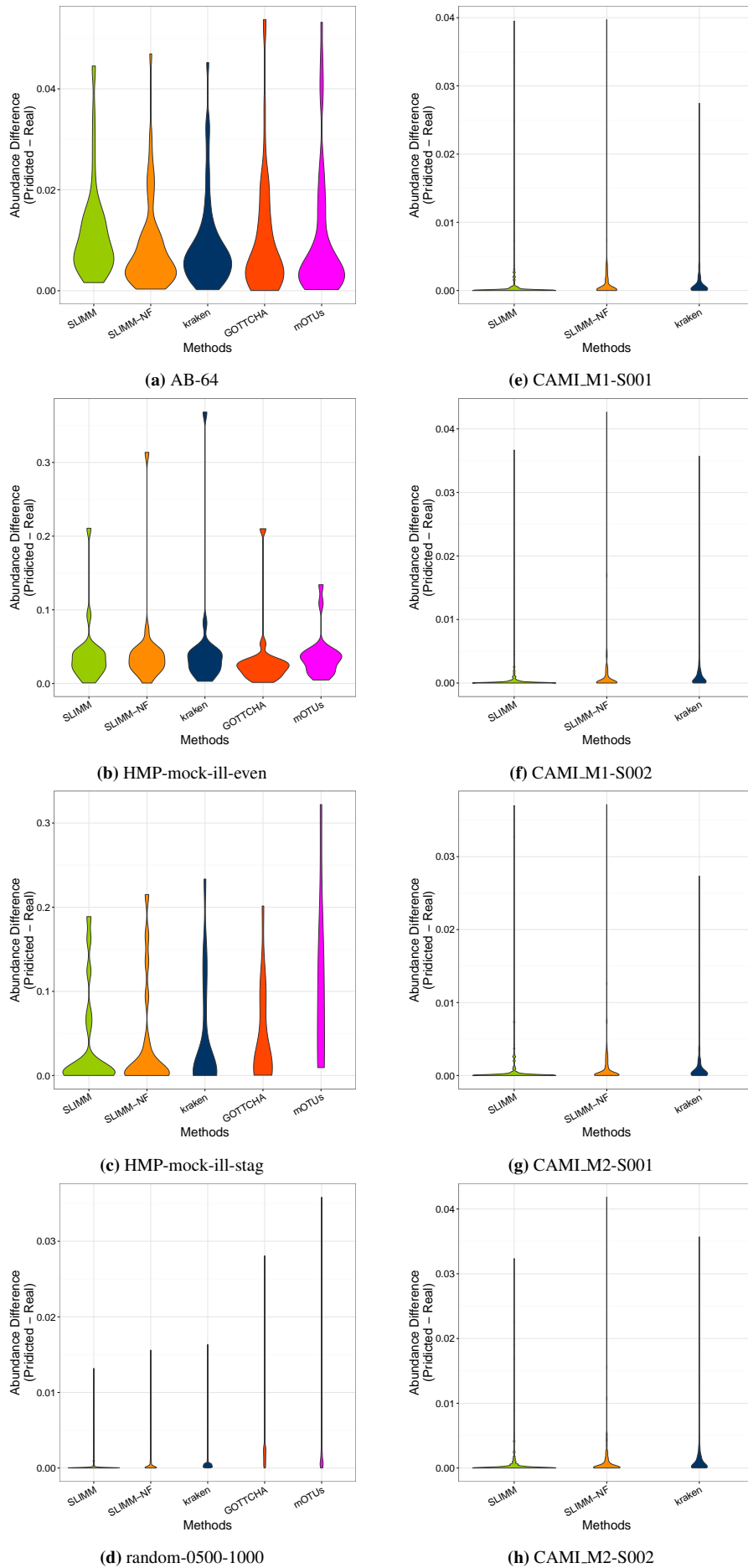
Figure 3. Violin Plots of the difference between real and predicted abundances: SLIMM vs Existing Methods
