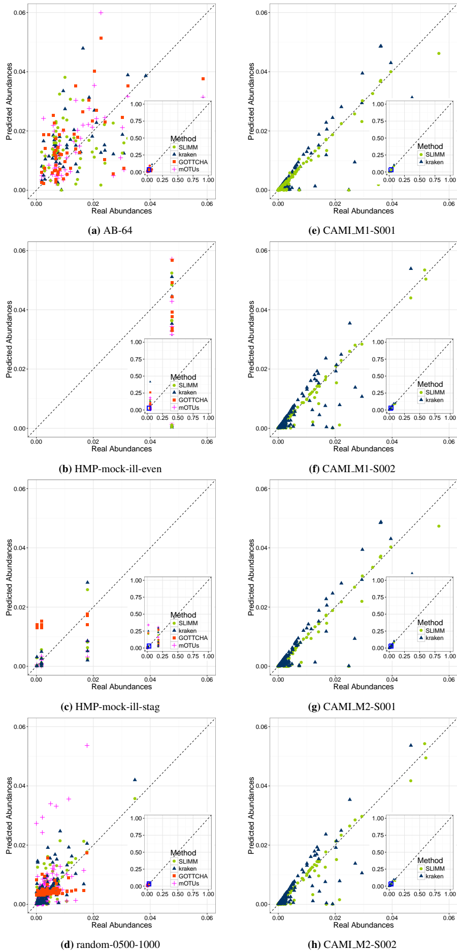
Figure 5. predicted vs real abundances: SLIMM vs Existing Methods
