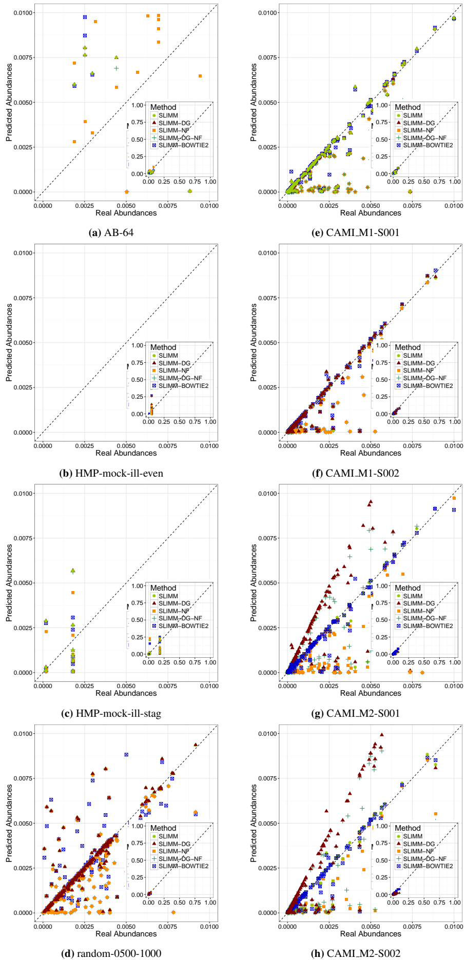
Figure 6. predicted vs real abundances: Different SLIMM variants
