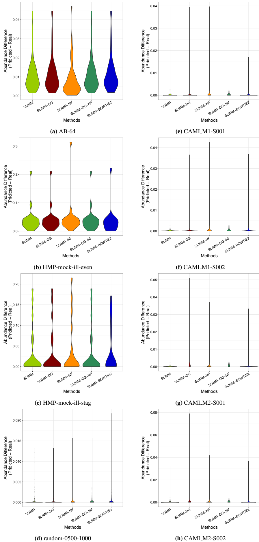
Figure 4. Violin Plots of the difference between real and predicted abundances: Different SLIMM variants
