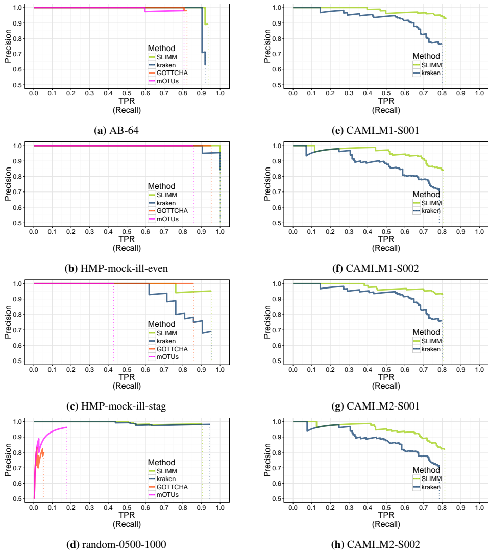
Figure 1. Precision - Recall Curves: SLIMM vs Existing Methods
